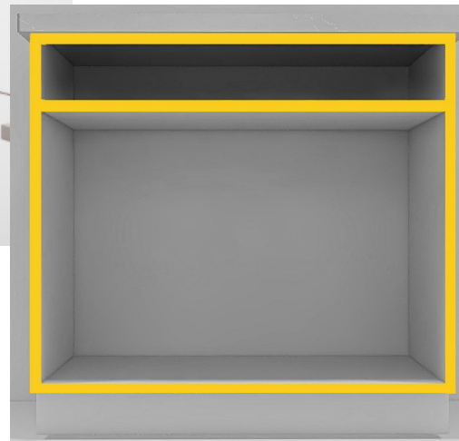
Frameless Cabinet Without Doors Made with 5/8" thick material.
